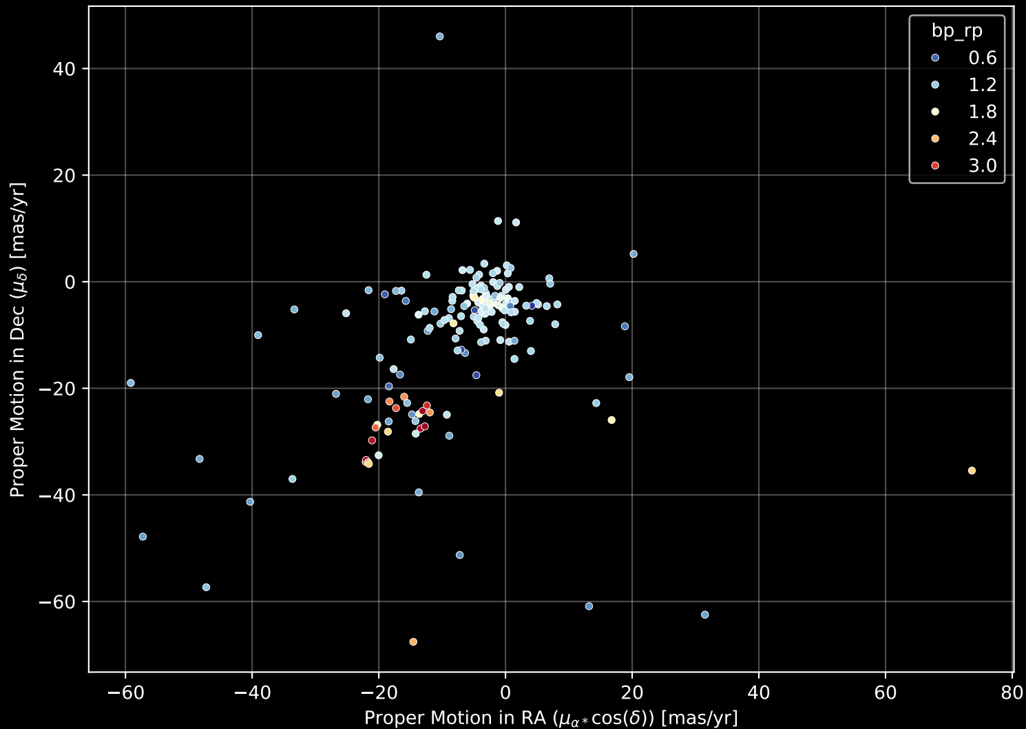
APOGEE DR17 Field: [347+20-O] Proper Motion Diagram (n= 171)
