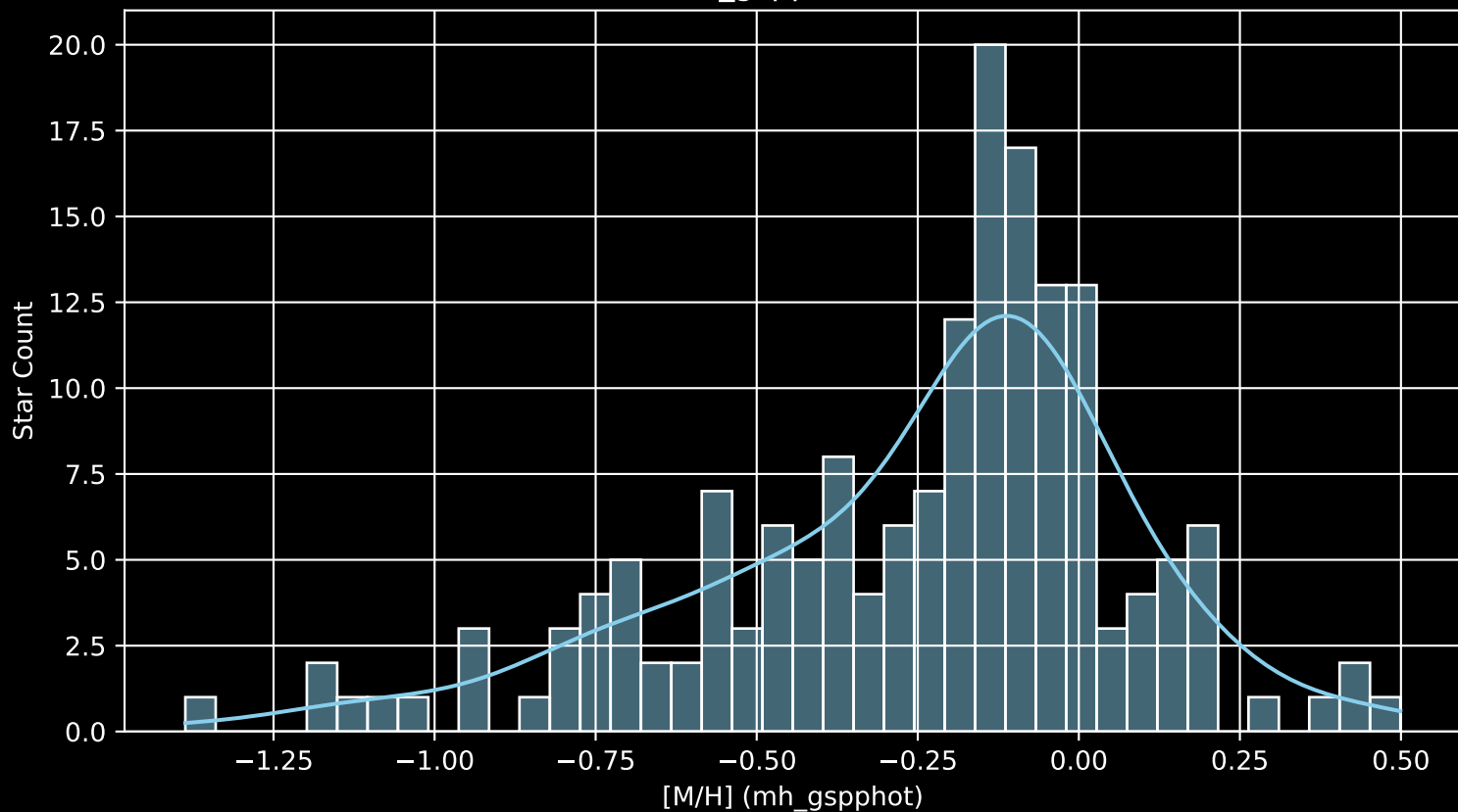
APOGEE DR17 Field: [347+20-O [M/H] (mh_gspphot) (n= 170)
