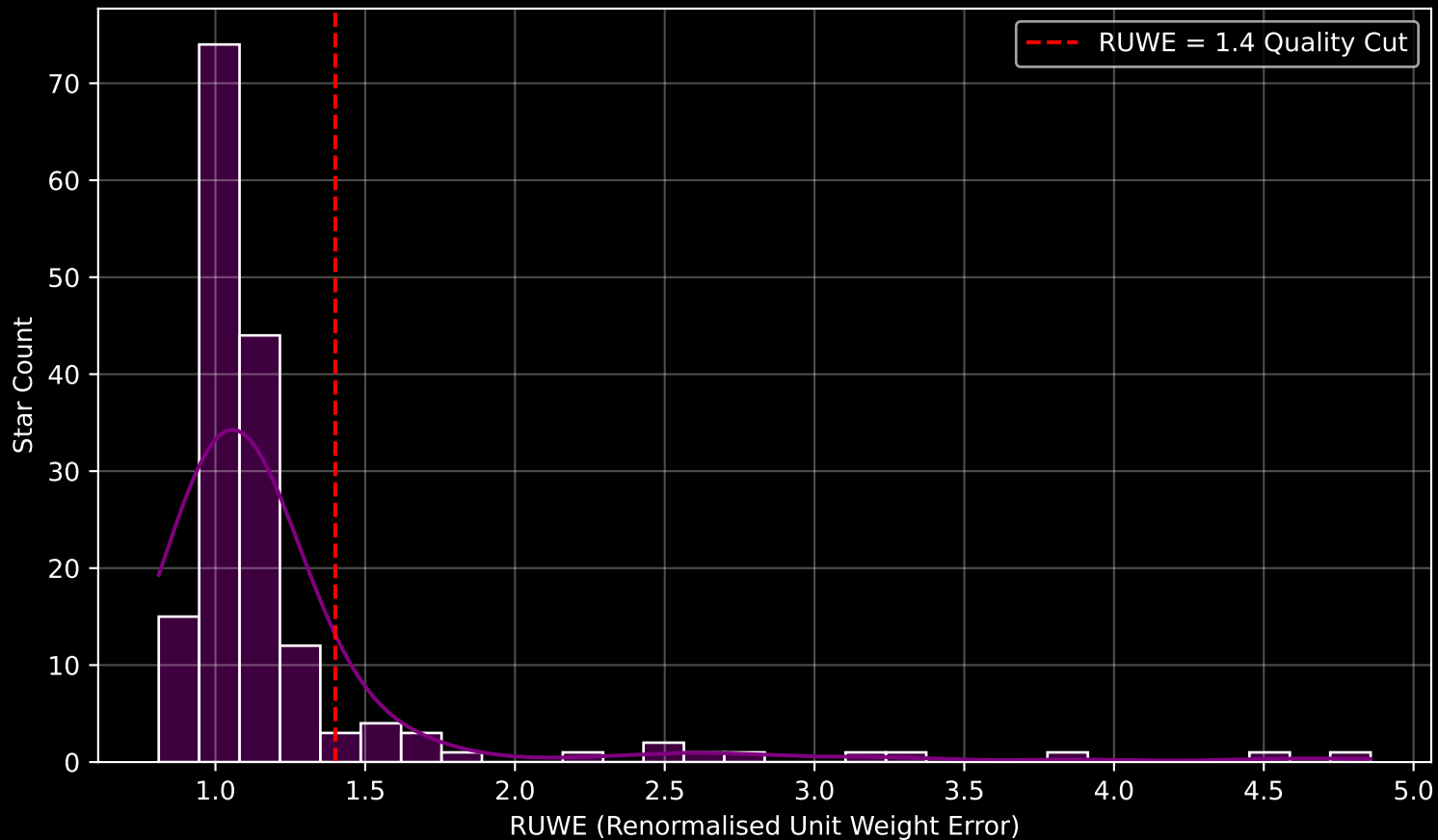
GAPOGEE DR17 Field [347+20-O] RUWE Distribution (n= 166)
