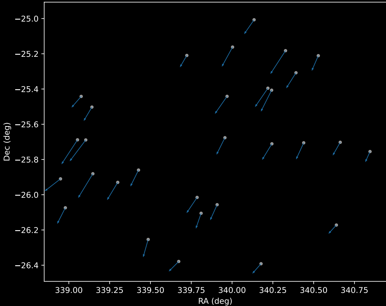
APOGEE DR17 Cluster 0 Proper Motion Vectors (n=30)
