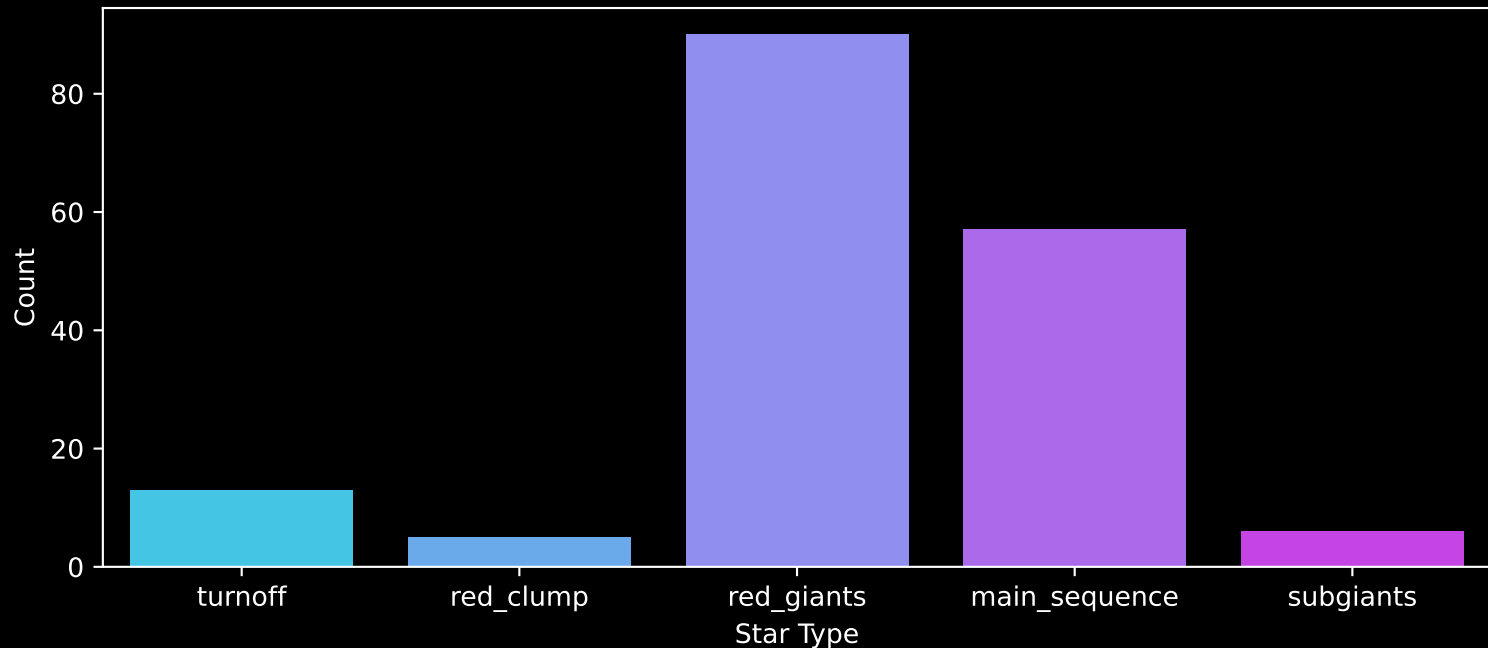
APOGEE DR17 Field: [347+20-O] Count plot of Star Type
