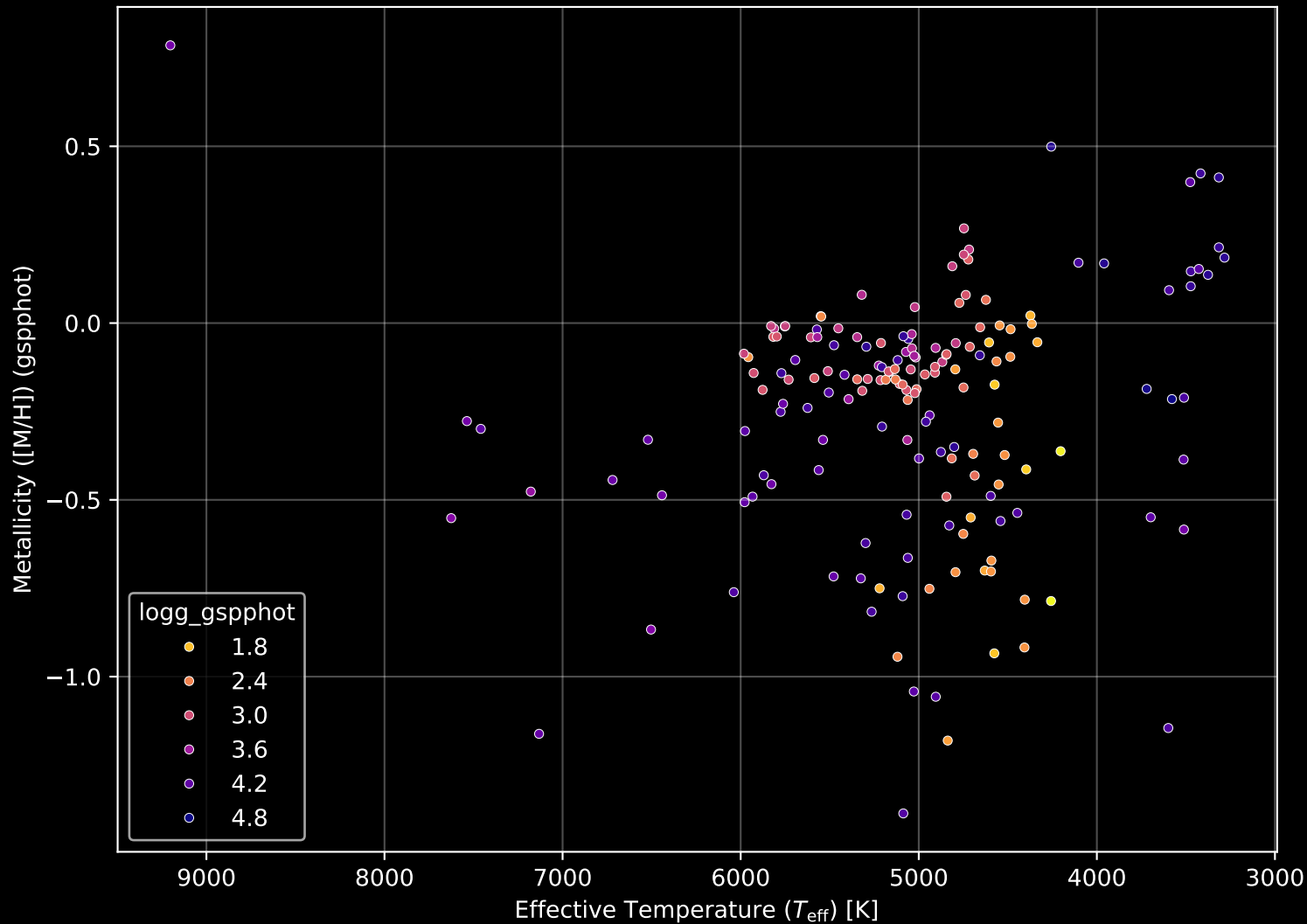
APOGEE DR17 Field: [347+20-O] Stellar Population Parameters (n= 171)
