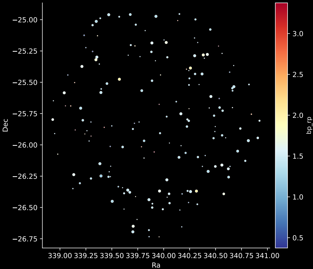
APOGEE DR17 Field: [347+20-O] Stars: 171
