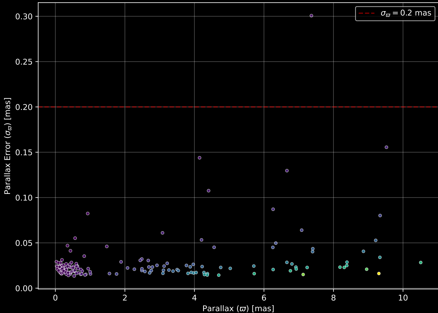
APOGEE DR17 Field: [347+20-O] Parallax Quality (n= 171)
